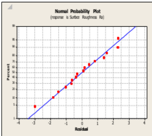
Figure 6 (c) Residual plots for fitted value
