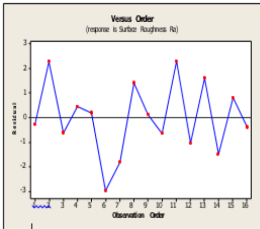
Figure 6 (a) Residual plot for Ra
